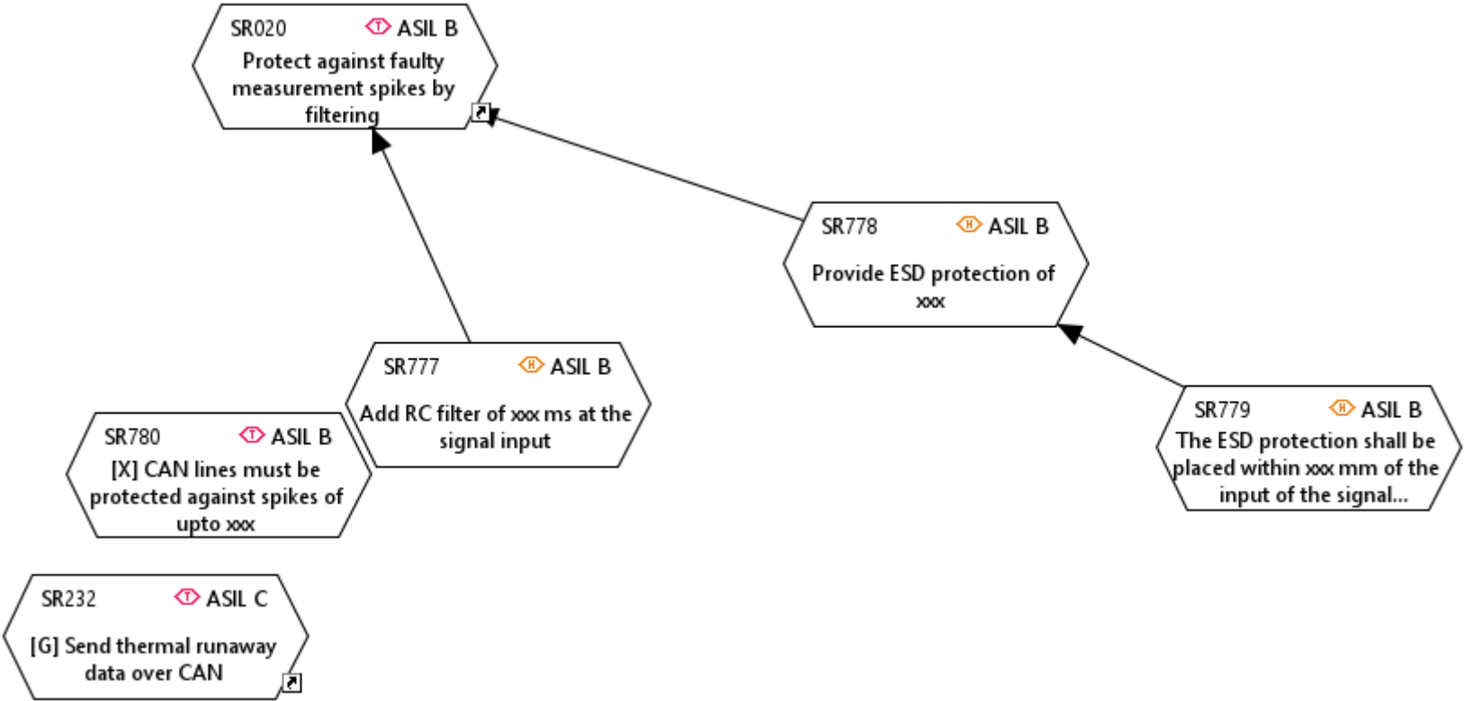
Figure 3.1: HW Safety Concept
